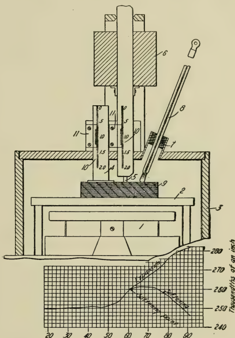
FIG. 195.—Apparatus for Determining the Softening-point of Bituminized Aggregates.
